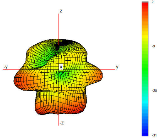
Typical 3D Pattern- Cell B - 750 MHz
